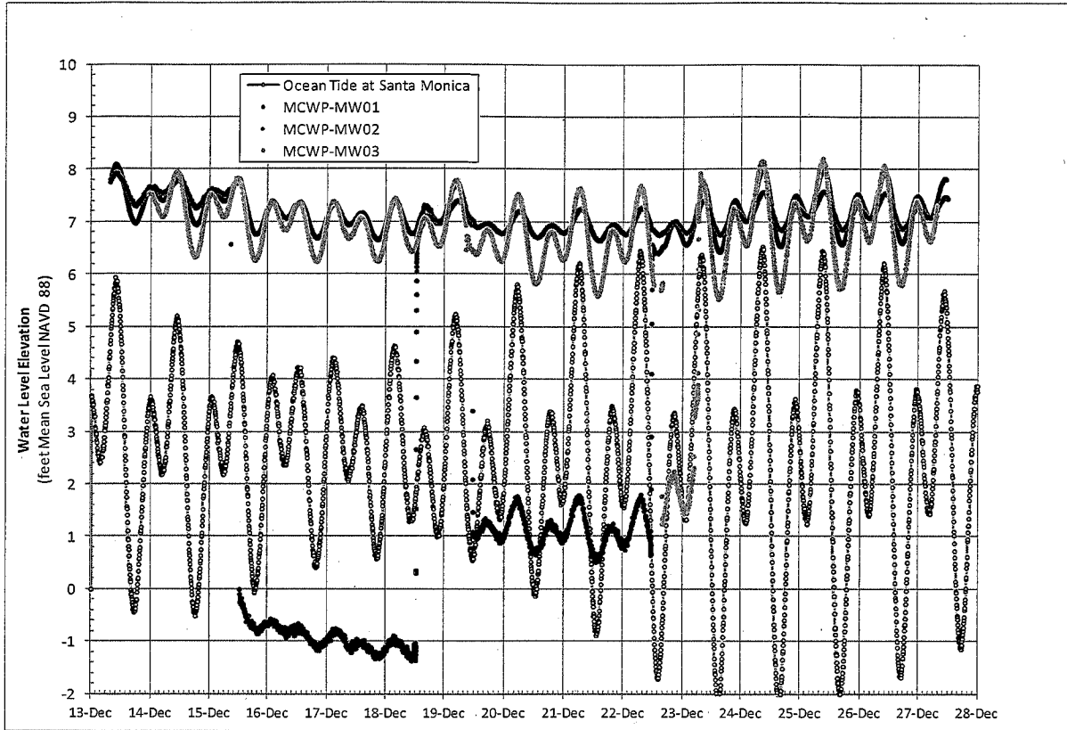
Figure 3.2- Water Level Elevation at New Test Wells (NAVD88)
